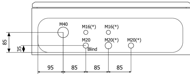
CABINET BOTTOM VIEW
