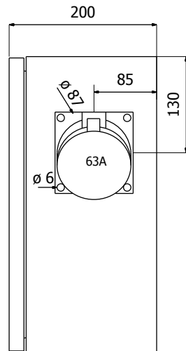
CABINET RIGHTHAND VIEW
